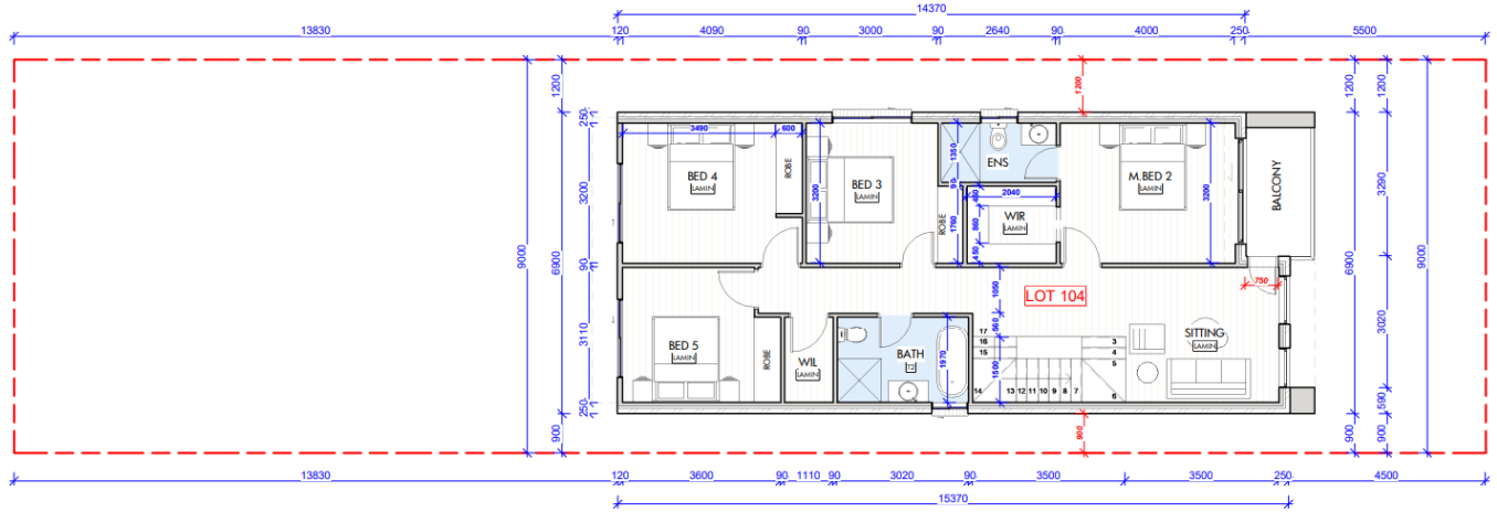
FIRST FLOOR
