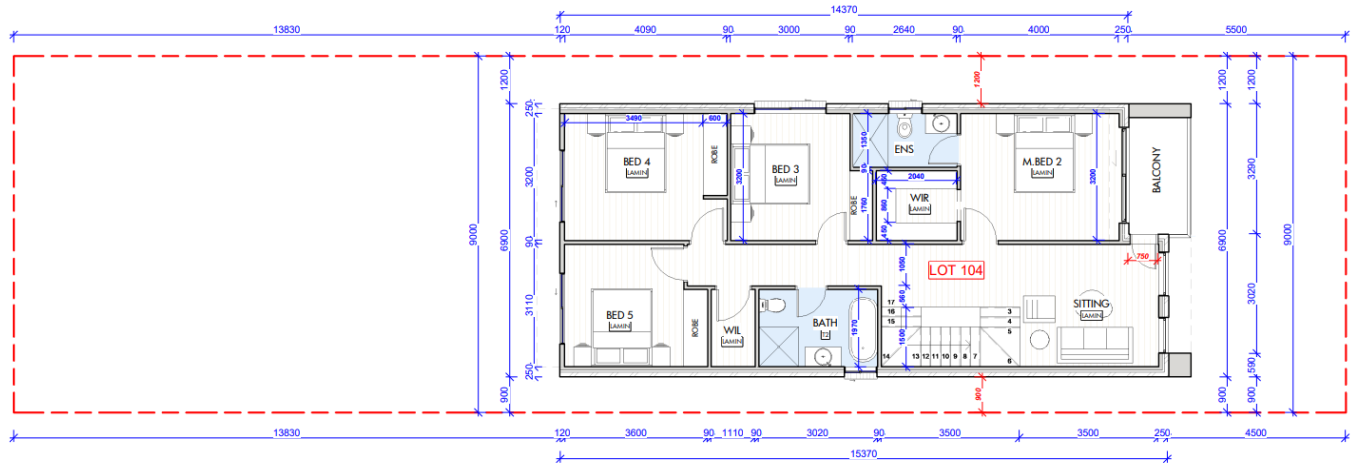
FIRST FLOOR
